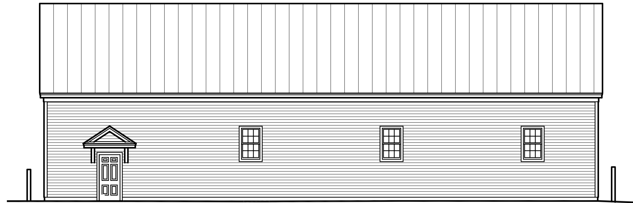
NORTH ELEVATION 1/8" = 1'-0"
